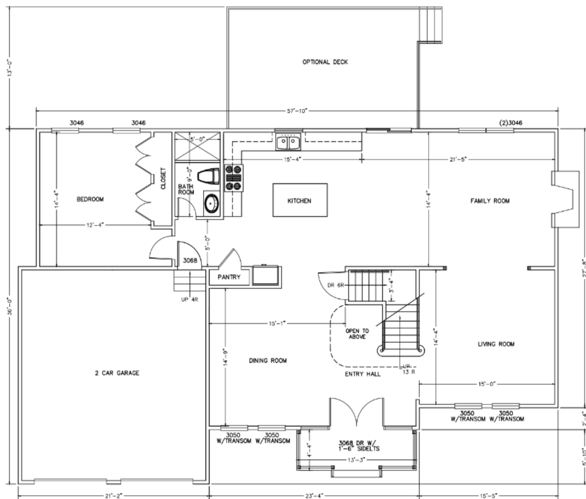
FIRST FLOOR PLAN 1502 SQ. FT.
