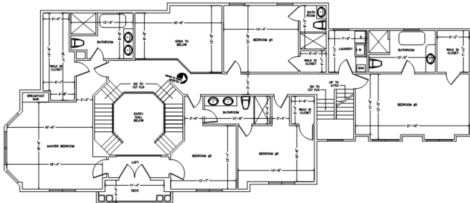
SECOND FLOOR PLAN 2366 SQ. FT.
