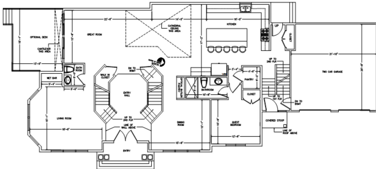
FIRST FLOOR PLAN 2080 SQ. FT.
